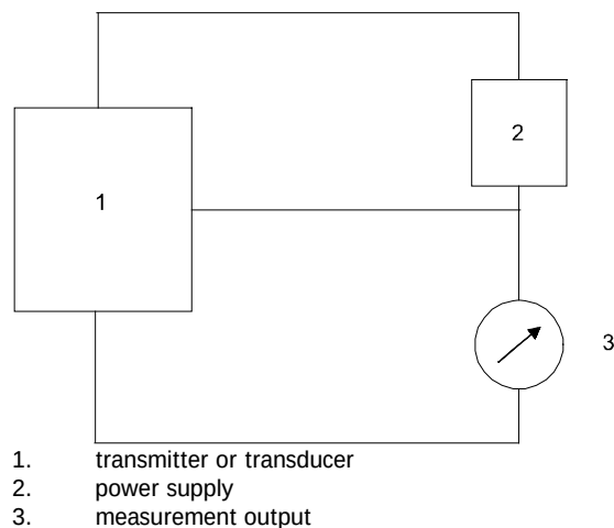
Figure 5 - Electrical set-up, three-wire transmitters or transducers
